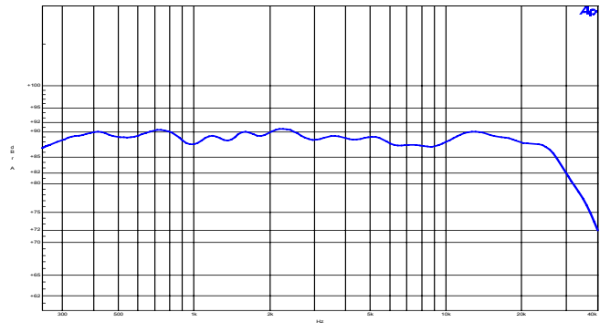
Frequency- response \pm 1,5 dB: Mid- high range
