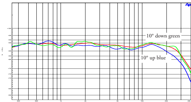
Frequency response: nearly no interferences, horizontal \pm 10^\circ
