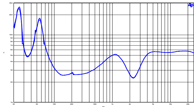
Loudspeaker: Impedance curve
