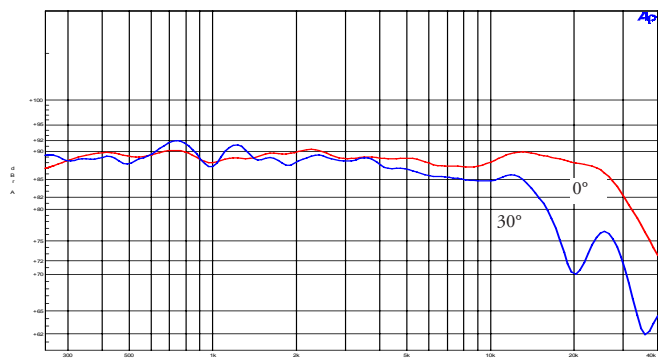
Frequency response: Also -30° out of axe vertical, very linear, excellent listening angle with APC. MK 3- System.
